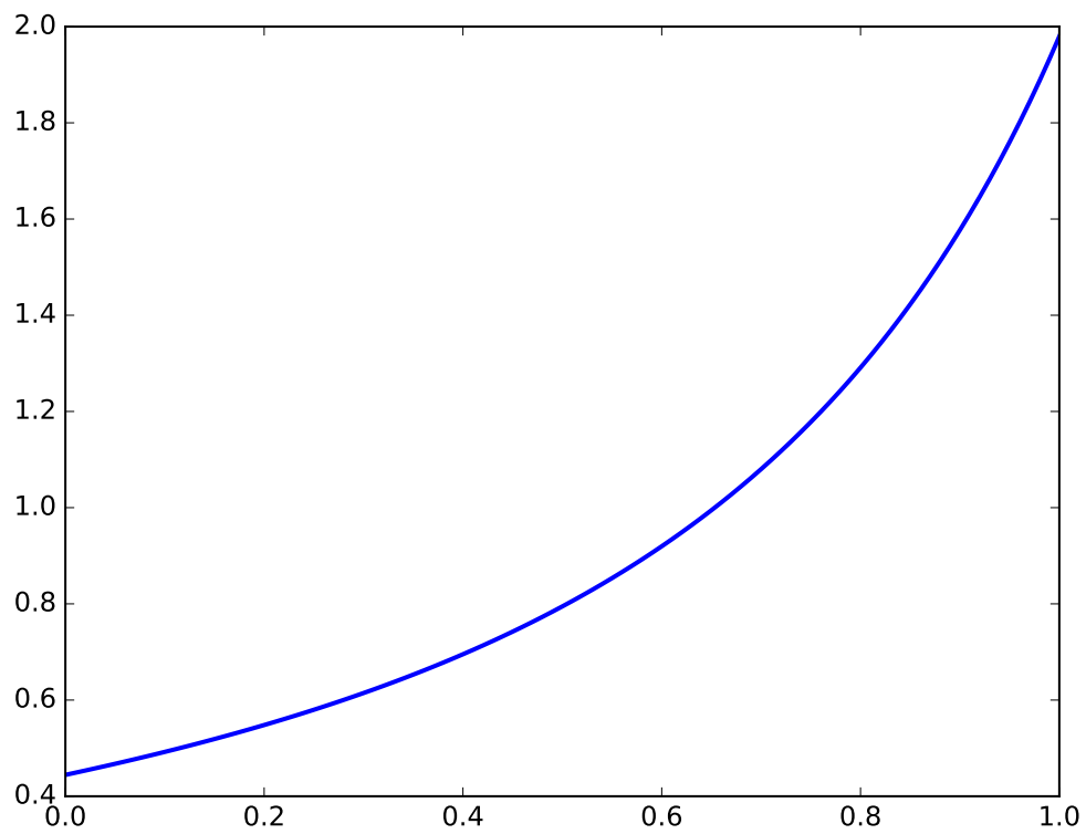
Figure 1.3: The density function a(x) satisfying (1.5) for \varepsilon = .8 .
