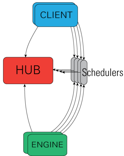
Figure 1.1: An outline of the iPyParallel architecture.
