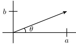
Figure 1.3: Rotating clockwise by \theta sends the vector [a, b]^\top to the span of \mathbf{e}_1 .
