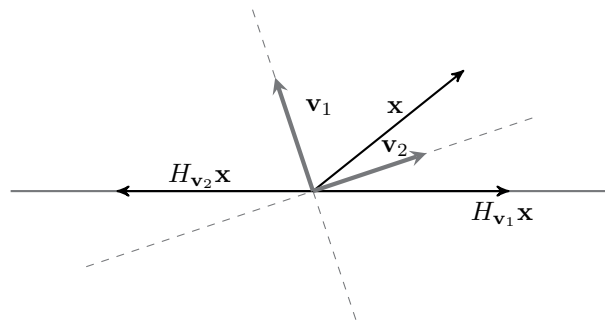
Figure 1.2: There are two reflections that map \mathbf{x} into the span of \mathbf{e}_1 , defined by the vectors \mathbf{v}_1 and \mathbf{v}_2 . In this illustration, H_{\mathbf{v}_2} is the more stable transformation since it reflects \mathbf{x} further than H_{\mathbf{v}_1} .
