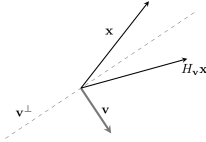
Figure 1.1: The vector \mathbf{v} defines the orthogonal complement \mathbf{v}^\perp , which in this case is a line. Applying the Householder transformation H_{\mathbf{v}} to \mathbf{x} reflects \mathbf{x} across \mathbf{v}^\perp .
