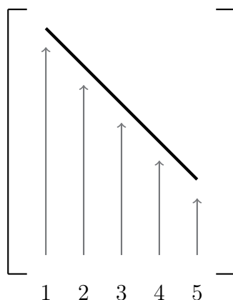
Figure 1.4: The order in which to zero out subdiagonal entries in the Givens triangularization algorithm. The heavy black line is the main diagonal of the matrix. Entries should be zeroed out from bottom to top in each column, beginning with the leftmost column.
