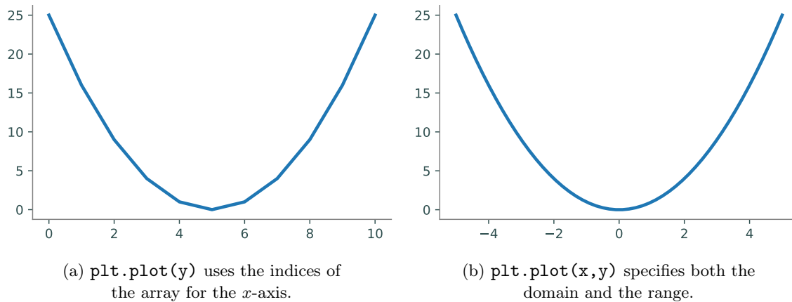
Figure 1.1: Plots of f(x) = x^2 over the interval [-5, 5] .
