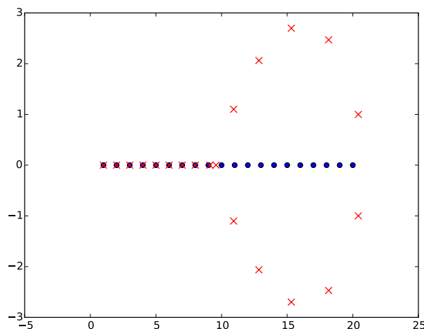
Figure 17.1: The blue dots are the roots of w(x) . The red dots are the roots of the polynomial perturbed by 1e-7 in the x^{19} -coefficient.
