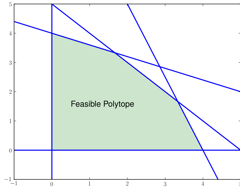
Figure 1.1: The feasible region for a linear program. The optimal point is one of the vertices of the polytope.
