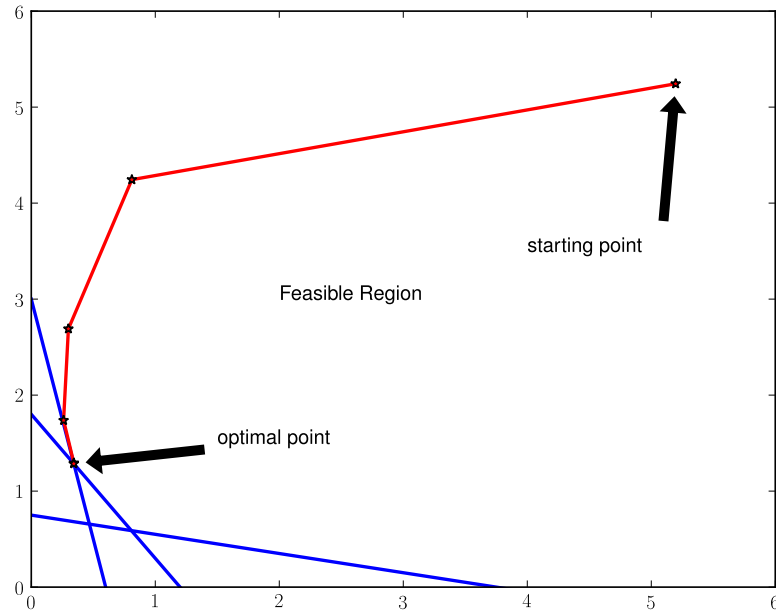
Figure 1.1: A path traced by an Interior Point algorithm.
