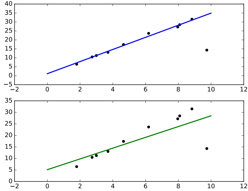
Figure 1.2: Fitted lines produced by least absolute deviations (top) and least squares (bottom). The presence of an outlier accounts for the stark difference between the two lines.
