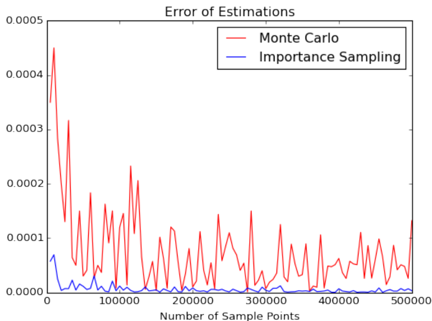
Figure 19.2: Comparison of error between standard method Monte Carlo and Importance Sampling method of Monte Carlo.
