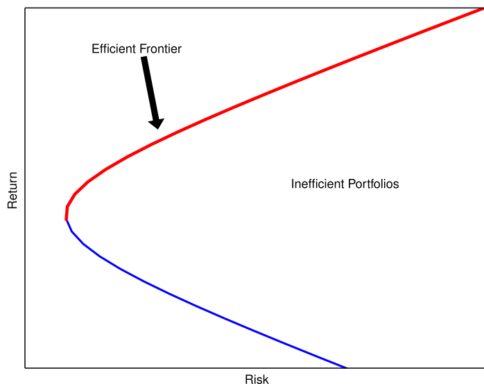
Figure 22.2: Efficient frontier on the risk-return plane.
