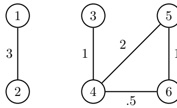
(b) G_2 , a weighted undirected graph.
