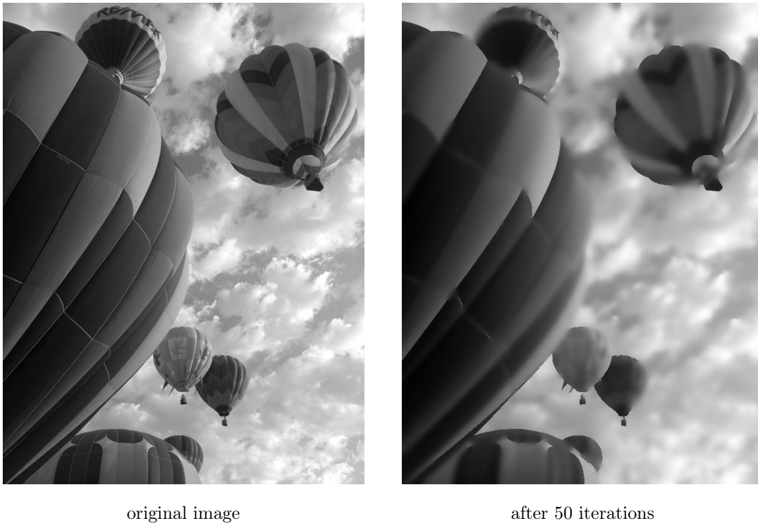
Figure 9.1: Smearing of similar colors when using an anisotropic diffusion filter.
