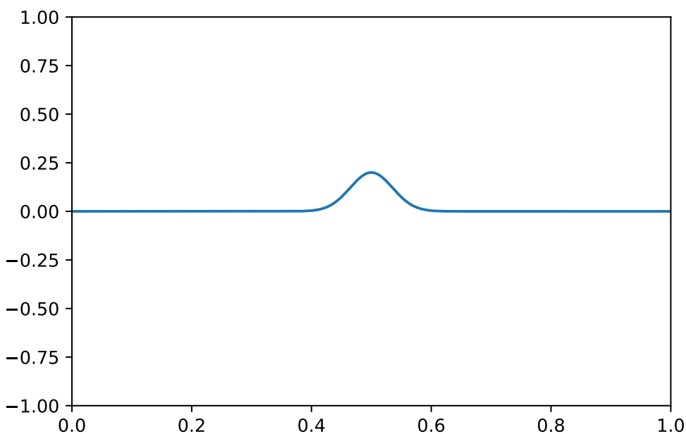
Figure 1.2: u(x, t = 0) .
