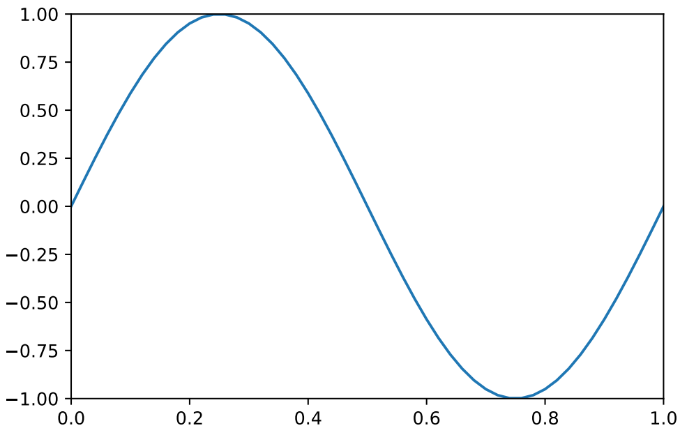
Figure 1.1: u(x, t = 0) .
