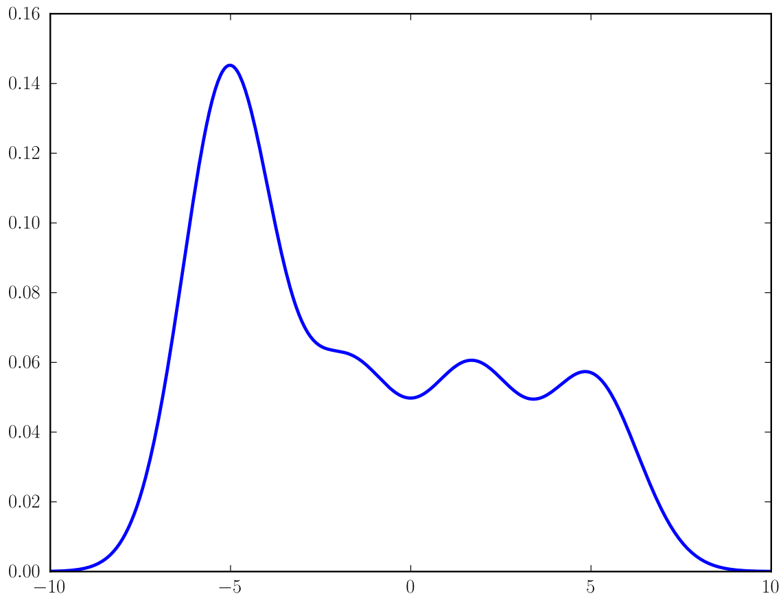
Figure 4.1: The probability density function of a mixture of Gaussians with four components.
