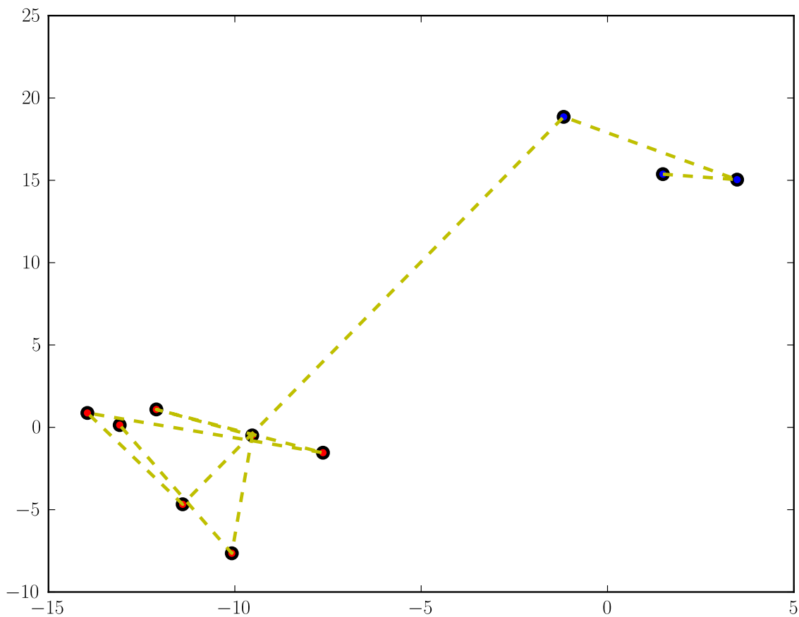
Figure 4.2: An observation sequence generated from a GMMHMM with one mixture component and two states. The observations (points in the plane) are shown as solid dots, the color indicating from which state they were generated. The connecting dotted lines indicate the sequential order of the observations.
