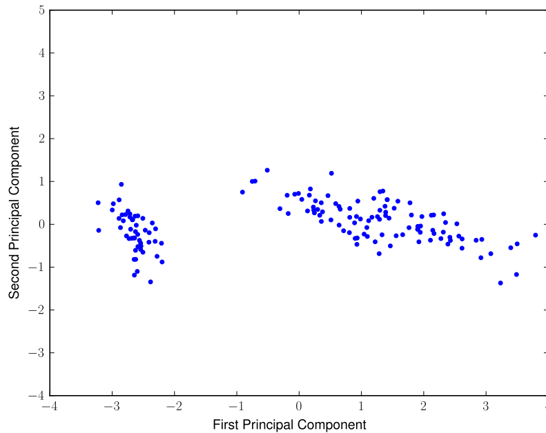
Figure 5.1: The first two principal components of the iris dataset.
