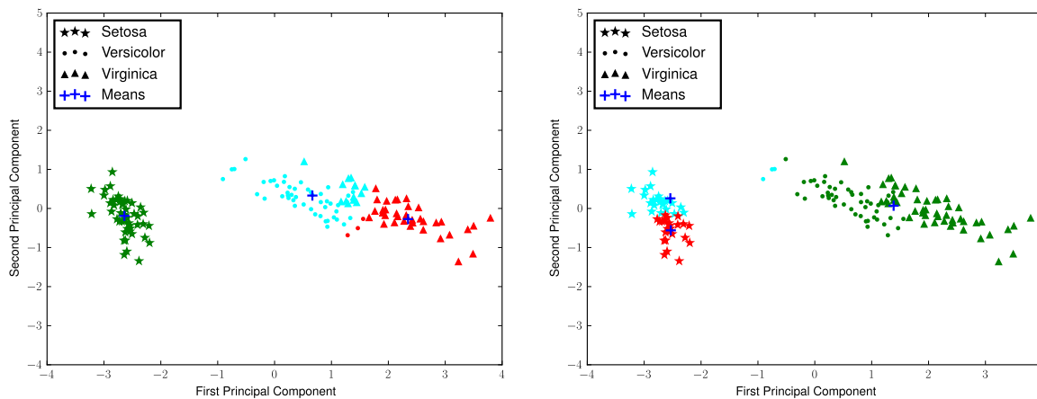
Figure 5.2: Two different K-Means clusterings for the iris dataset. Notice that the clustering on the left predicts the flower species to a high degree of accuracy, while the clustering on the right is less effective.
