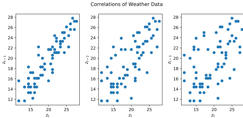
Figure 7.1: These graphs show that the weather data is correlated to its previous values. The correlation is weaker in each graph successively, showing that the further in the past the data is, the less correlated the data becomes.
