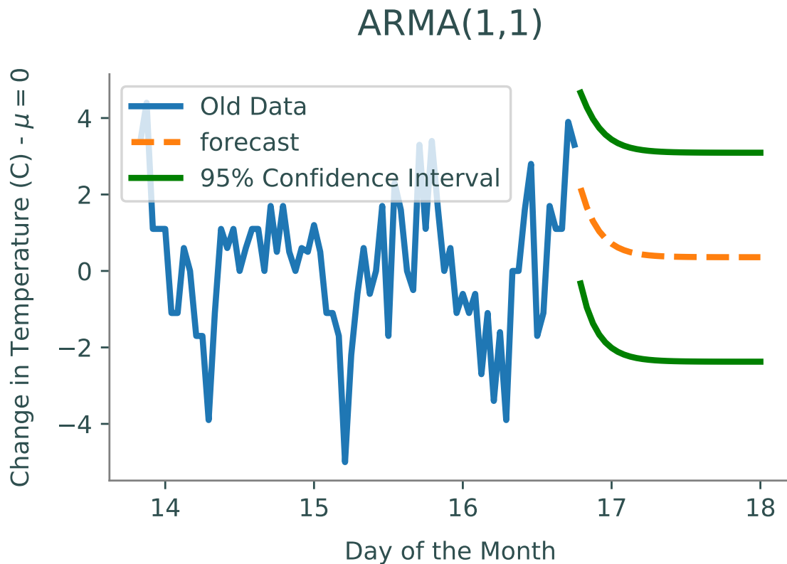
Figure 7.3: ARMA(1,1) forecast on weather.npy
