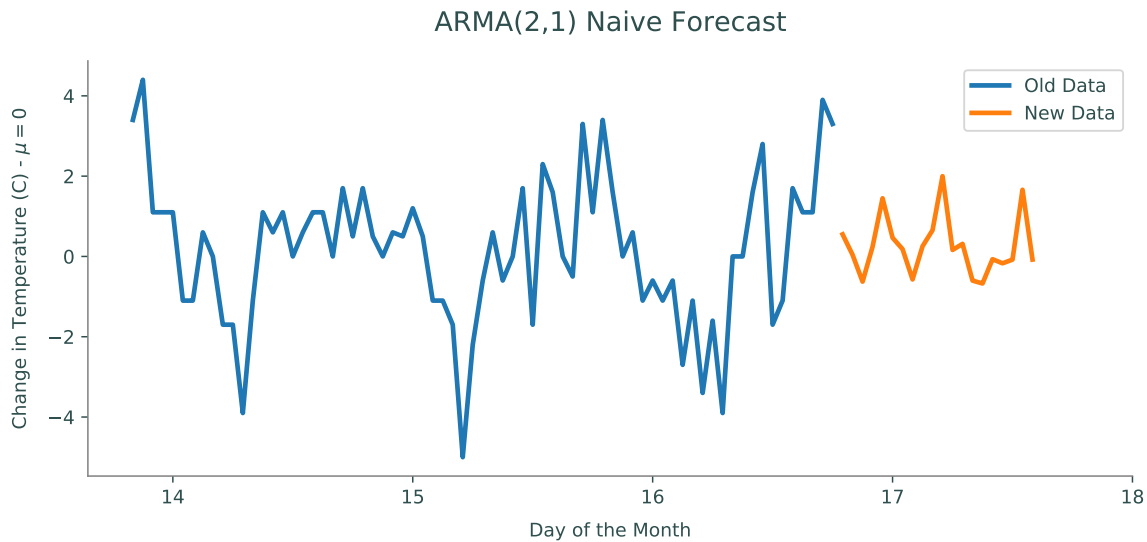
Figure 7.2: Naive forecast on weather.npy
