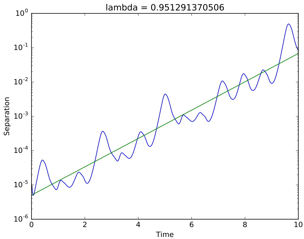
Figure 4.3: A semilog plot of the separation between two solutions to the Lorenz equations together with a fitted line that gives a rough estimate of the Lyapunov exponent of the system.
