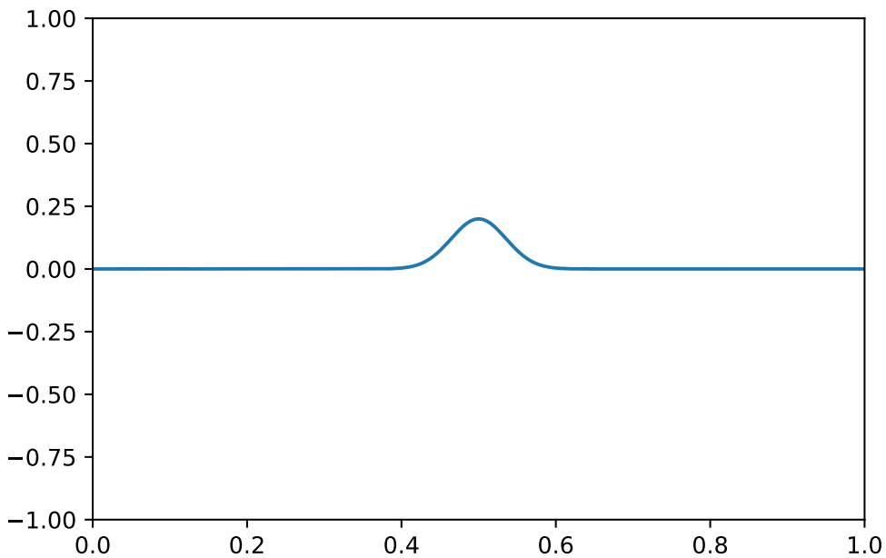
Figure 7.2: u(x, t = 0) .
