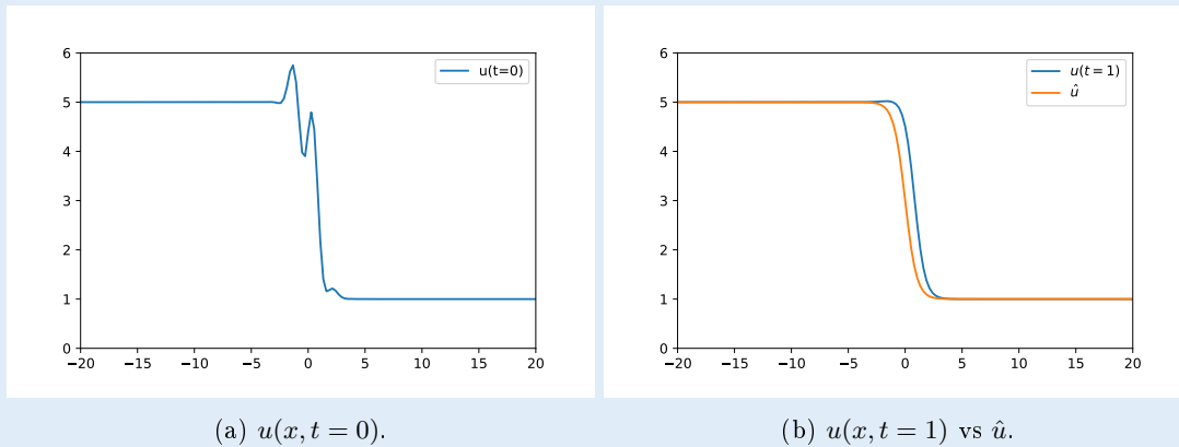
Figure 7.4: The graphs for Problem 5
