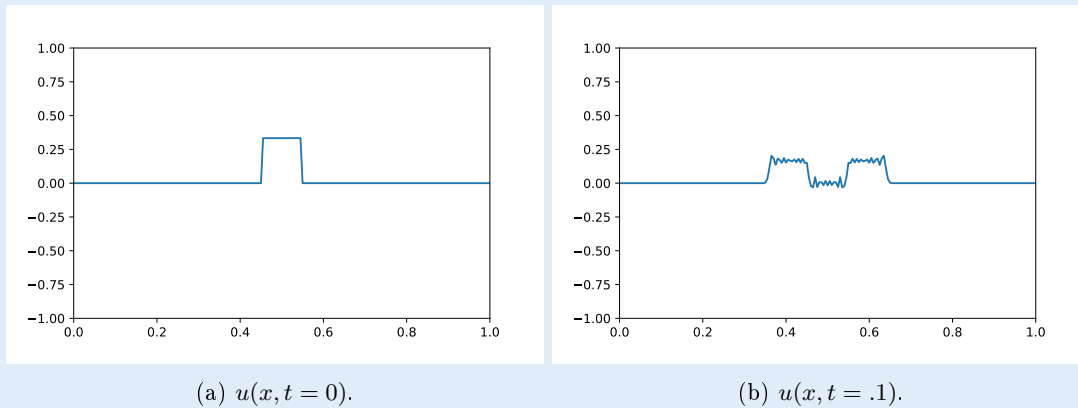
Figure 7.3: The graphs for Problem 4 at various times t .
