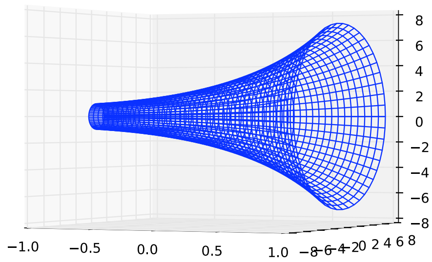
Figure 1.1: The minimal surface corresponding to Problem 5.
